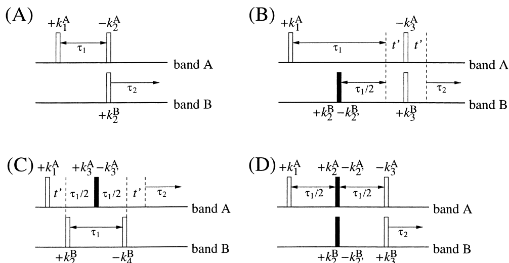
Fig. 4. Pulse sequences of important heteronuclear NMR experiments and building blocks for which optical analogs can be devised.
