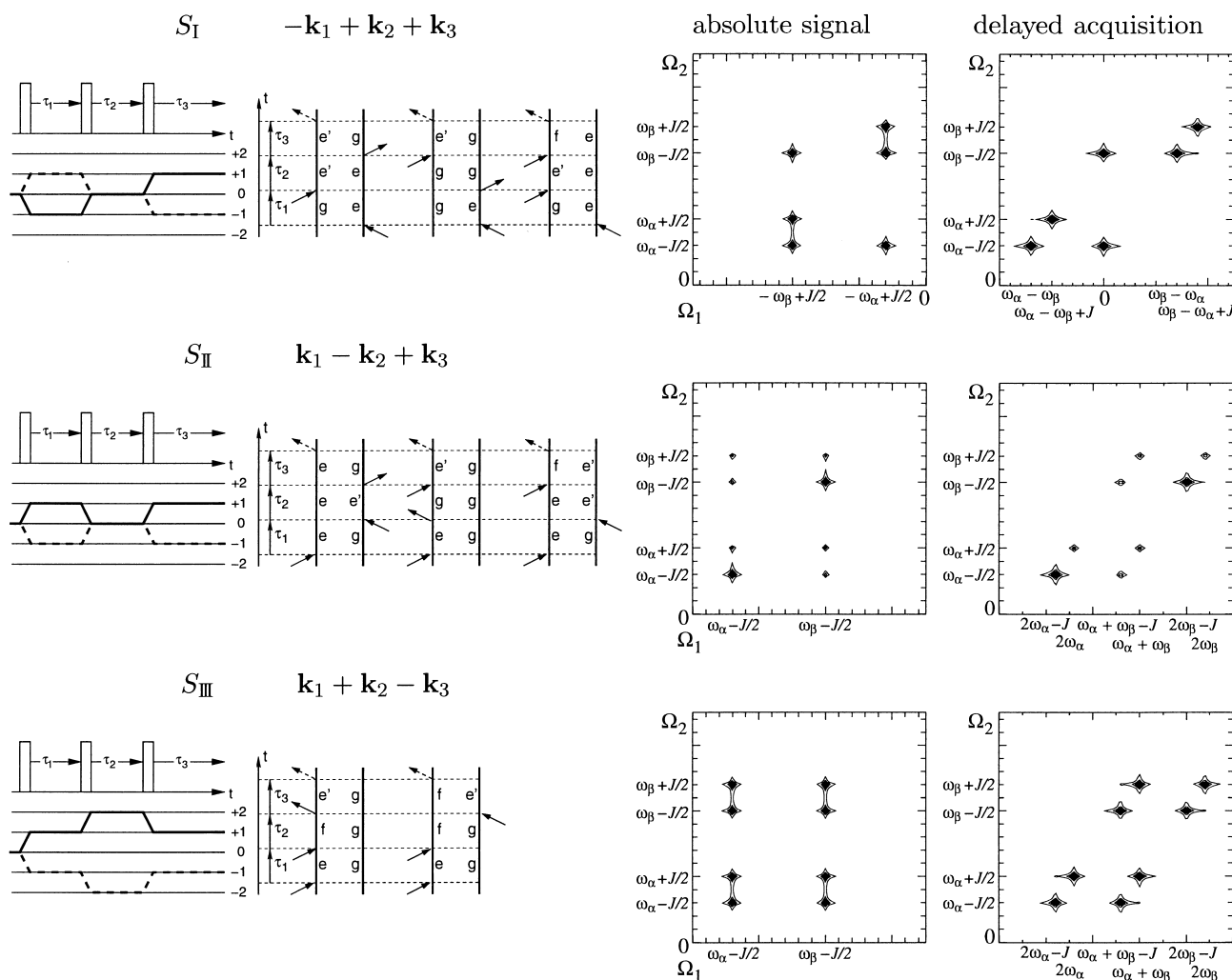
Fig. 1. The coherence order diagrams and double sided Feynman diagrams of the possible weak field signals from optical three-pulse experiments are shown along with the corresponding 2D absolute value spectra for a dimer of two-level systems. The frequency domains of the spectra are obtained by Fourier transformation of the time-delays \tau_1 and \tau_3 where \tau_2 = \tau_m is a short mixing time. The last column shows the signals for delayed acquisition with acquisition starting after an additional delay of \tau_1 after the third pulse. This is analogous to the detection in J -resolved spectroscopy and results in a skew transformation of the observed signals.
