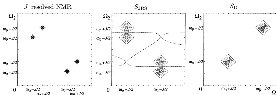
Fig. 3. Comparison of the NMR J -resolved experiment (without delayed acquisition) with the vibrational combination signal S_{JRS} that contains analogous information. In the complementary combination signal S_D only the diagonal peaks are retained.
