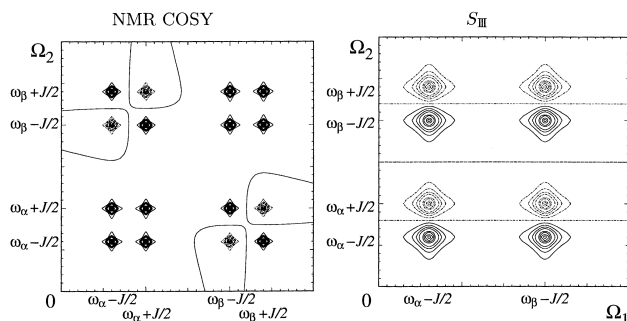
Fig. 2. Comparison of the NMR COSY experiment with the vibrational S_{\text{III}} three pulse signal that contains analogous information.
